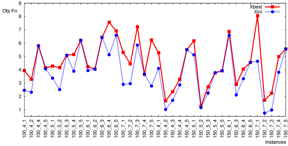
Figure 8: Comparison between the initial solution ( X^{ini} ) and the TS solution X^{best} for 100- to 150-BU instances.
