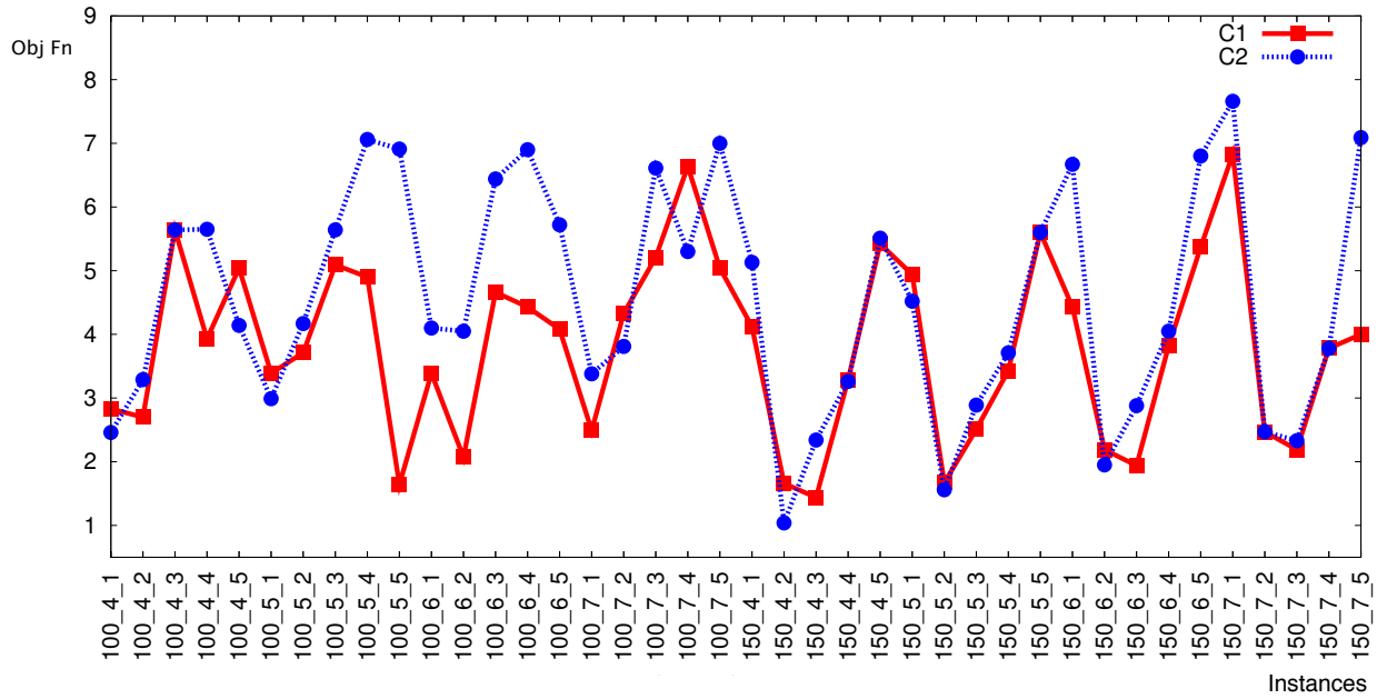
Figure 4: Objective function comparison between \mathcal{N}_{C1} and \mathcal{N}_{C2} on 100- and 150-BU instances.
